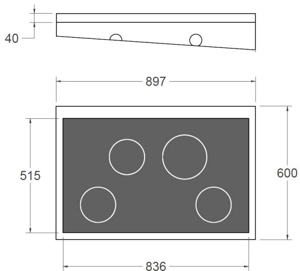
WORKTOP DETAILS
